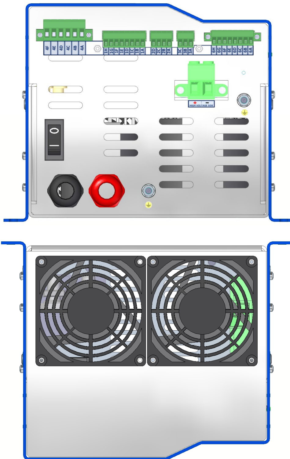
Fig. 1 DC/DC converter Size 1
